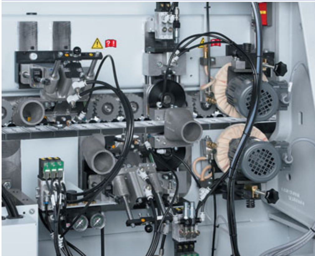
Profile scraping unit
